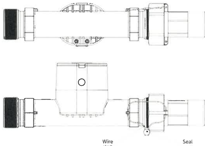
Fig. 2b) Sealing DN25 and DN32
