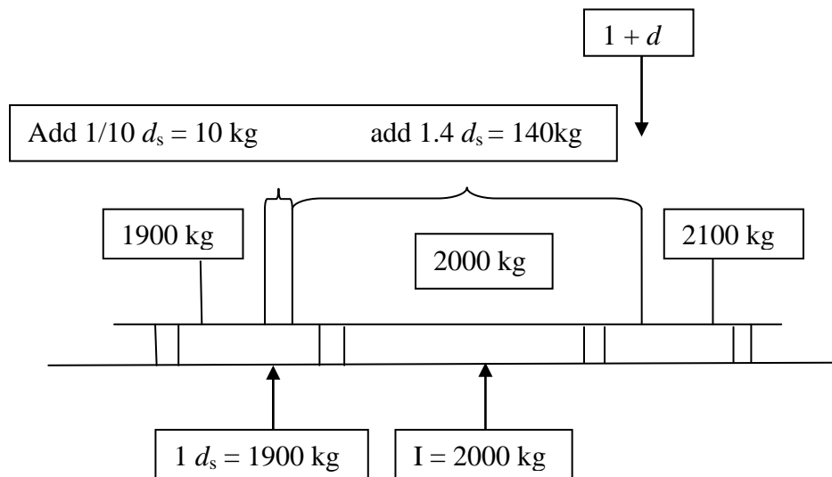
Figure 3 Example: Instrument with d_s = 100 kg
